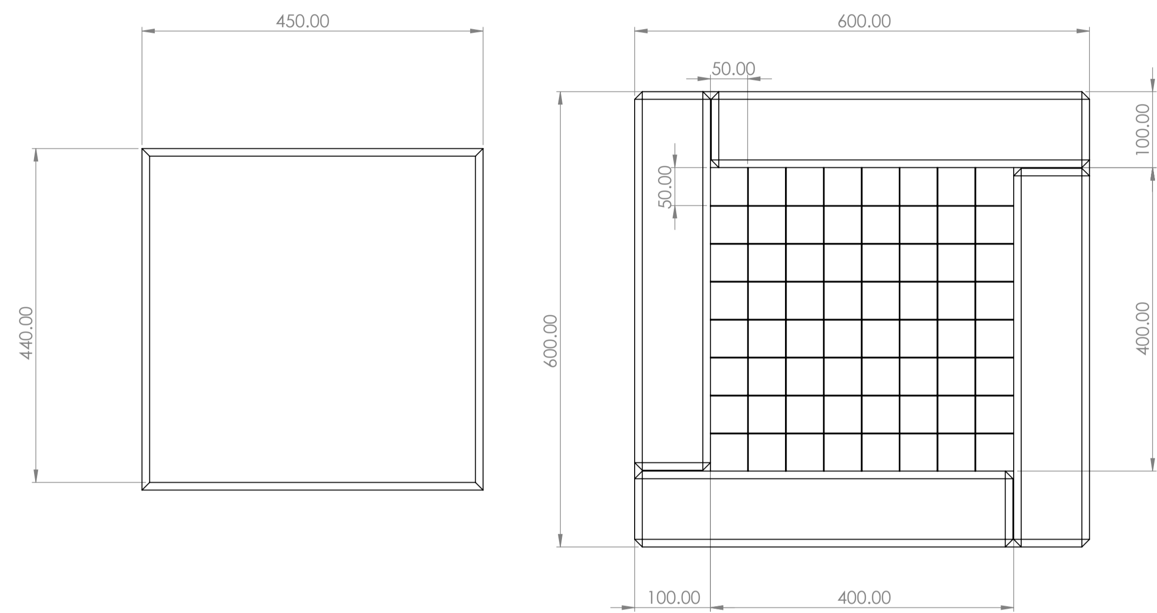
Plan View 1:5
