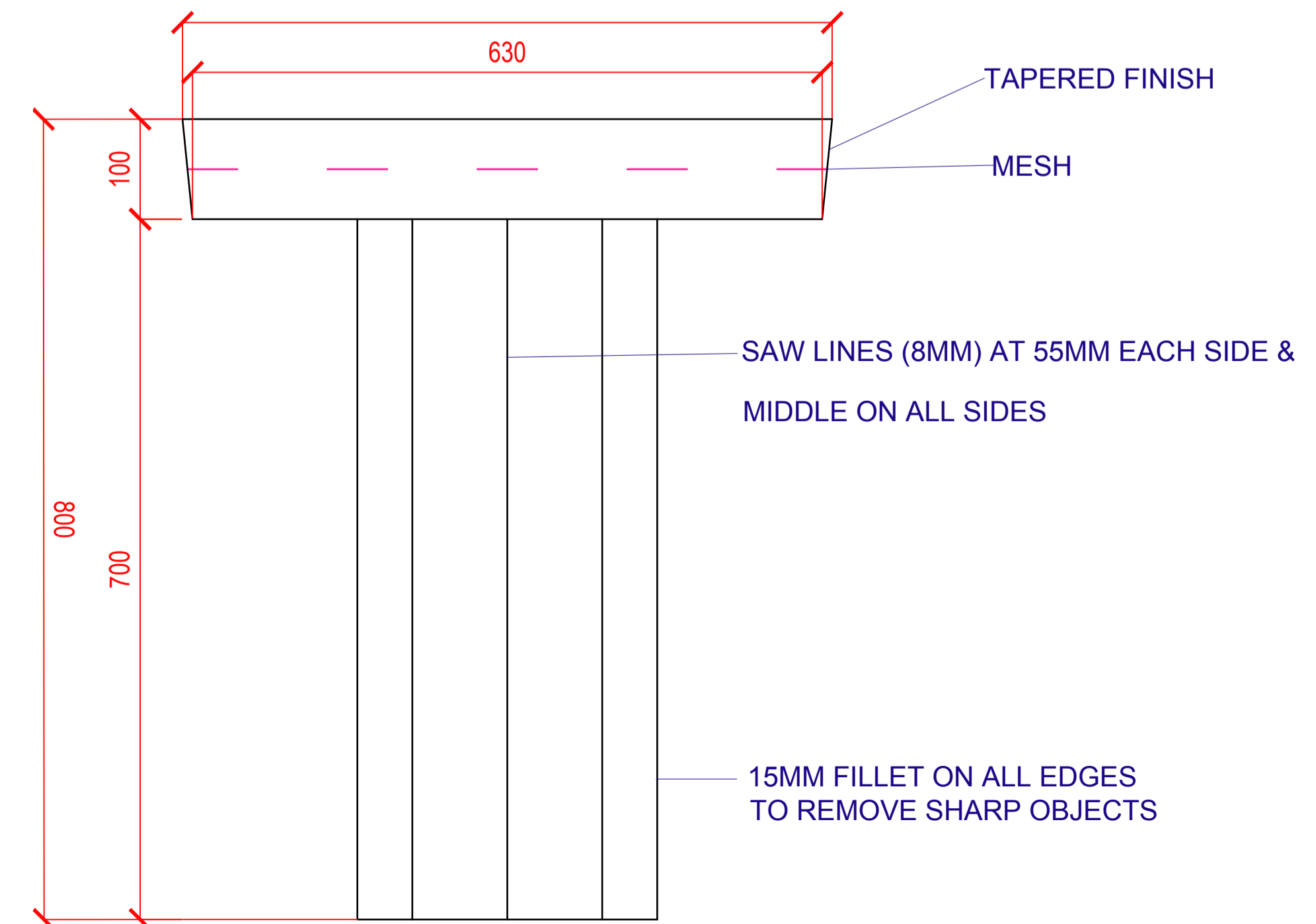
Front View 1:5
