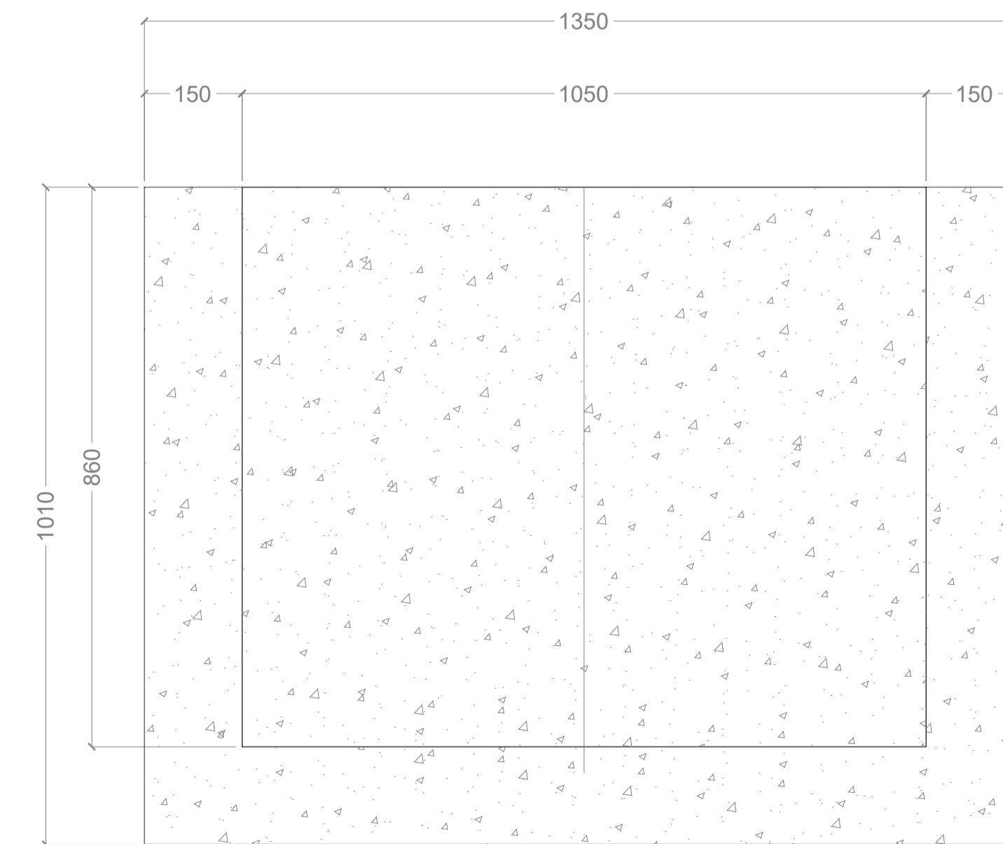
Detail 3: Planter Sectional View
